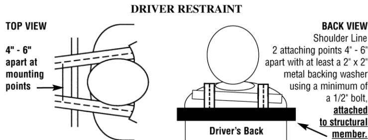
Figure 2 - Driver Restraint
